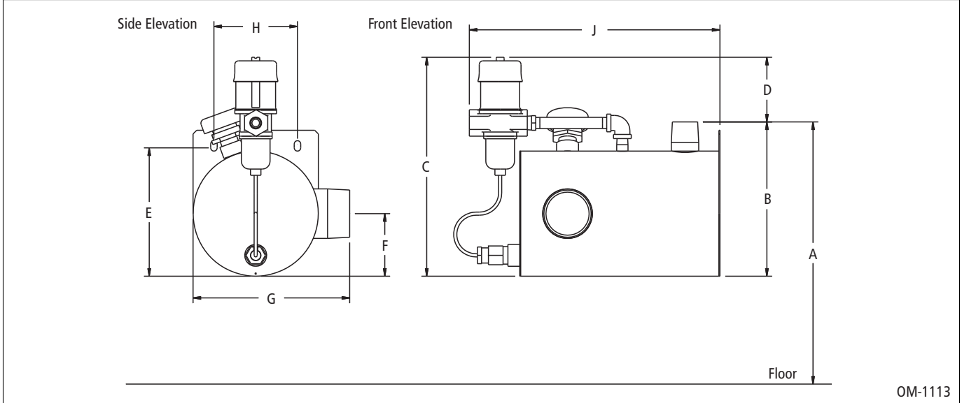
Figure 5-1: Drane-kooler dimensions
