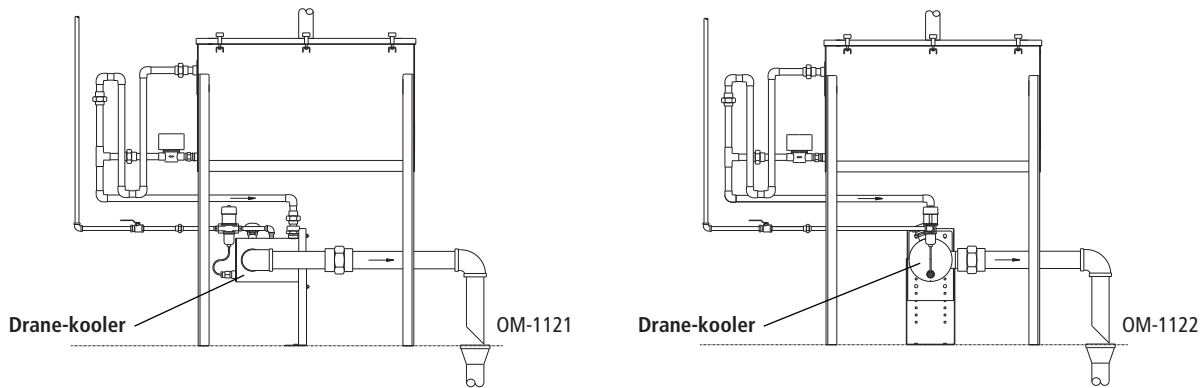
Figure 8-2: Drane-kooler mounted directly underneath an evaporative humidifier
